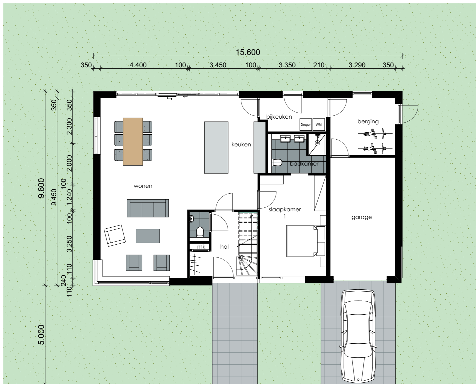
begane grond | 1:100
